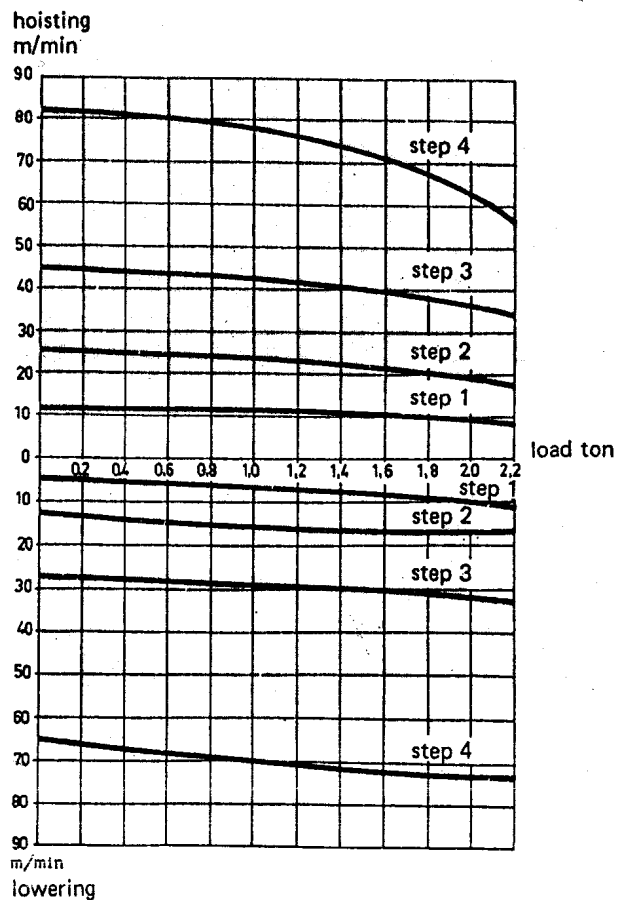
HOISTING/LOWERING SPEEDS in 4 steps
